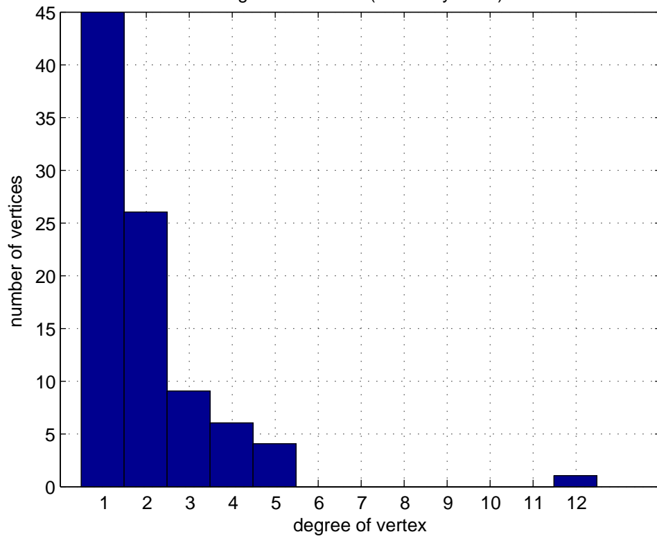
Degree of vertices (Germany 2006)
