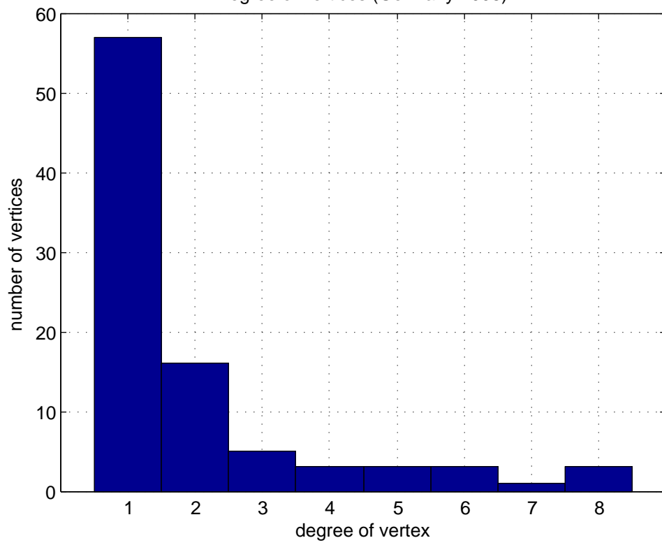
Degree of vertices (Germany 2008)
