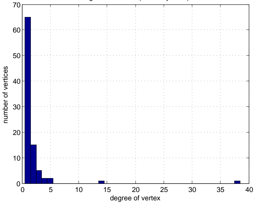
Degree of vertices (Germany 2005)
