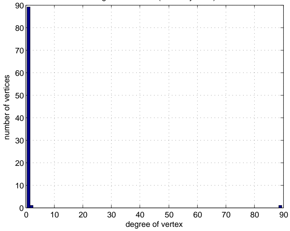
Degree of vertices (Germany 2004)
