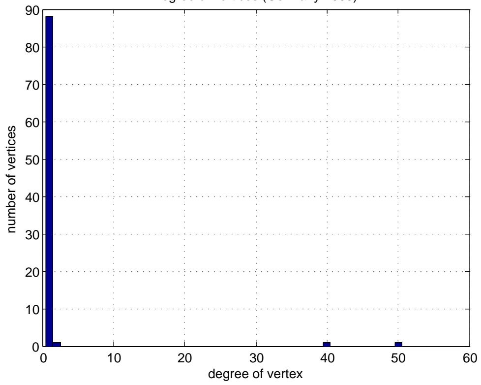
Degree of vertices (Germany 2003)
