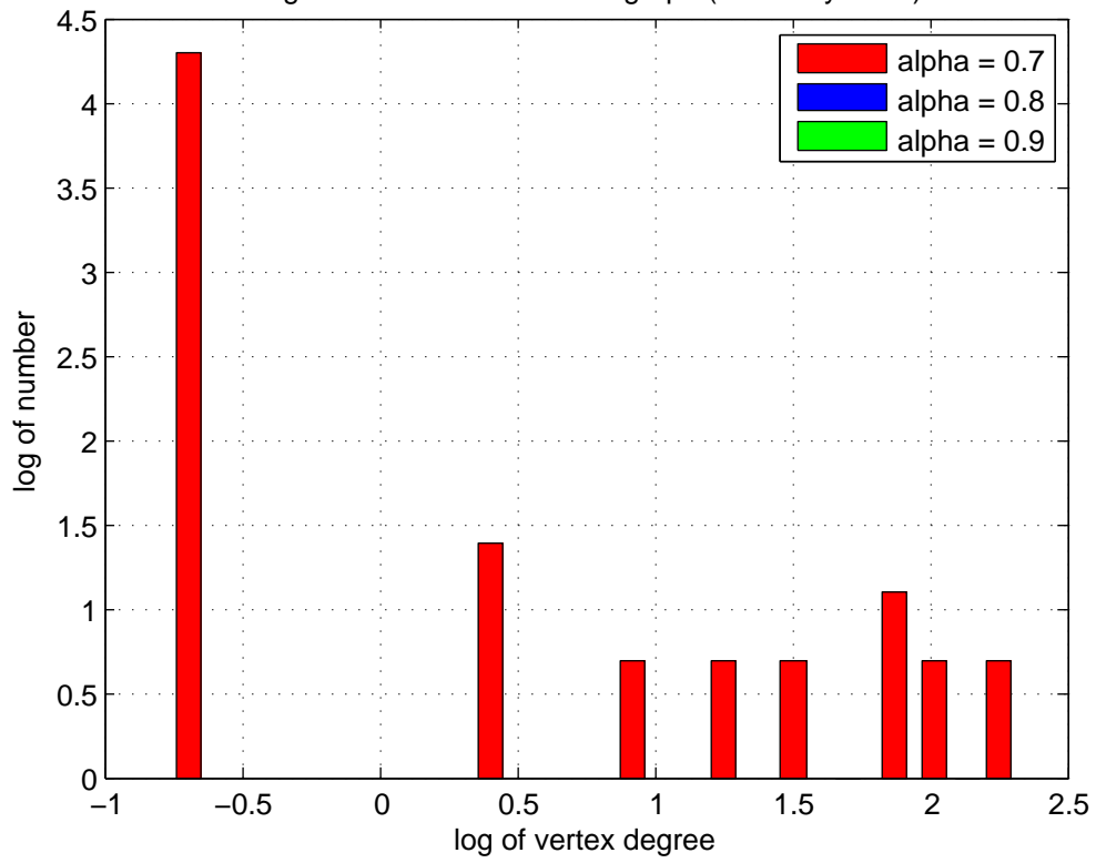
Degree of vertices in market graph (Germany 2005)
