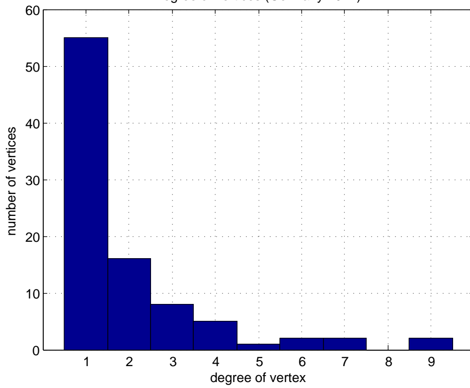
Degree of vertices (Germany 2011)
