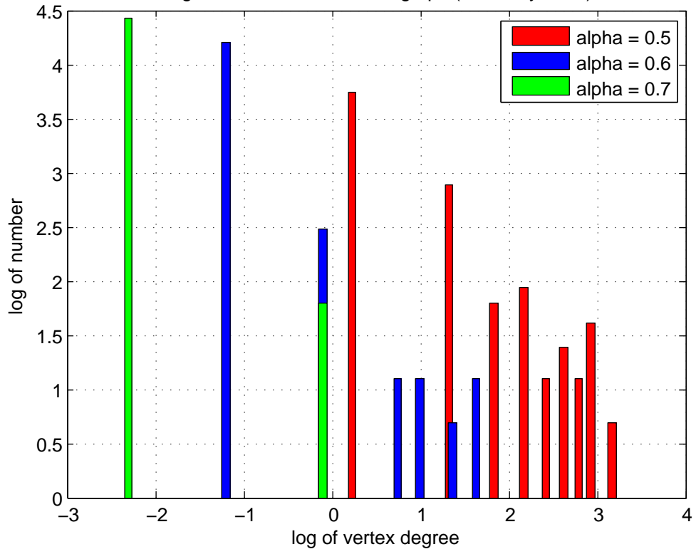
Degree of vertices in market graph (Germany 2013)
