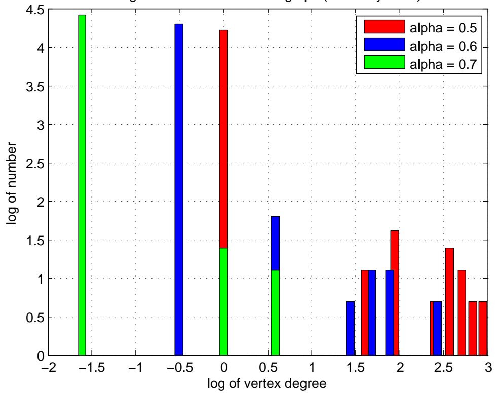
Degree of vertices in market graph (Germany 2004)
