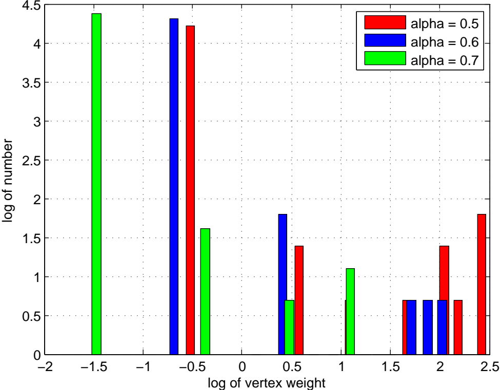
Weights of vertices in market graph (Germany 2003)
