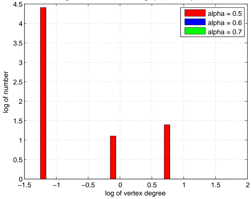
Degree of vertices in market graph (Germany 2014)
