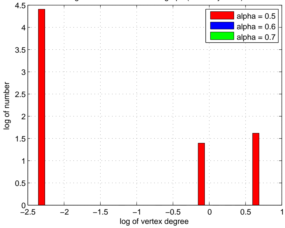
Degree of vertices in market graph (Germany 2009)
