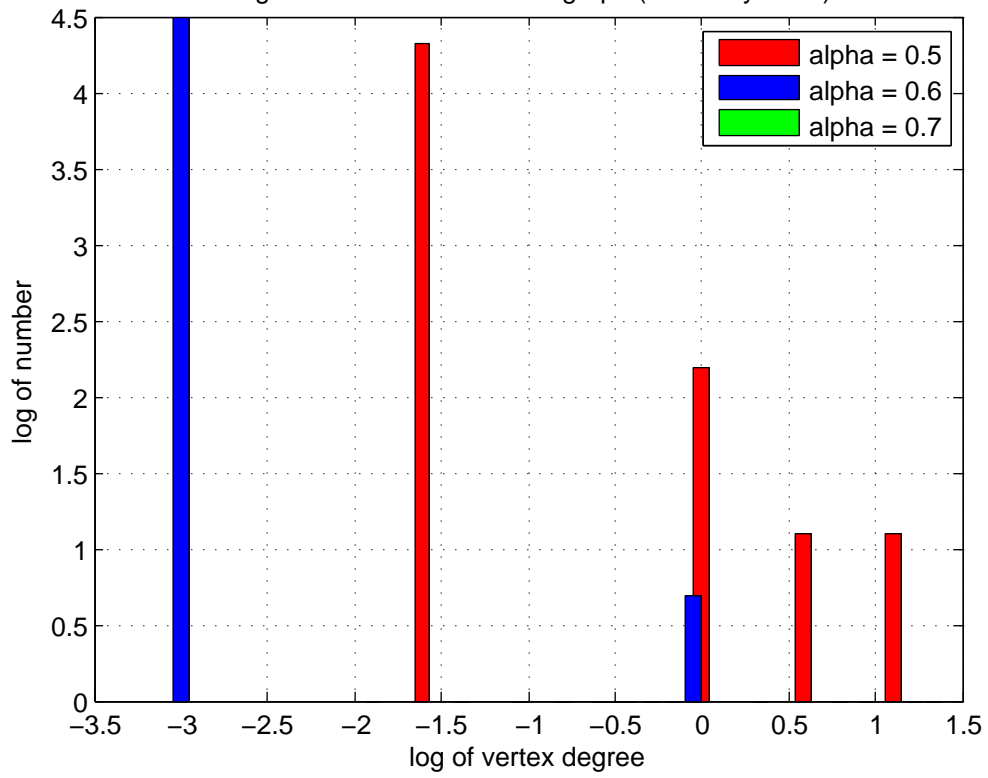
Degree of vertices in market graph (Germany 2012)
