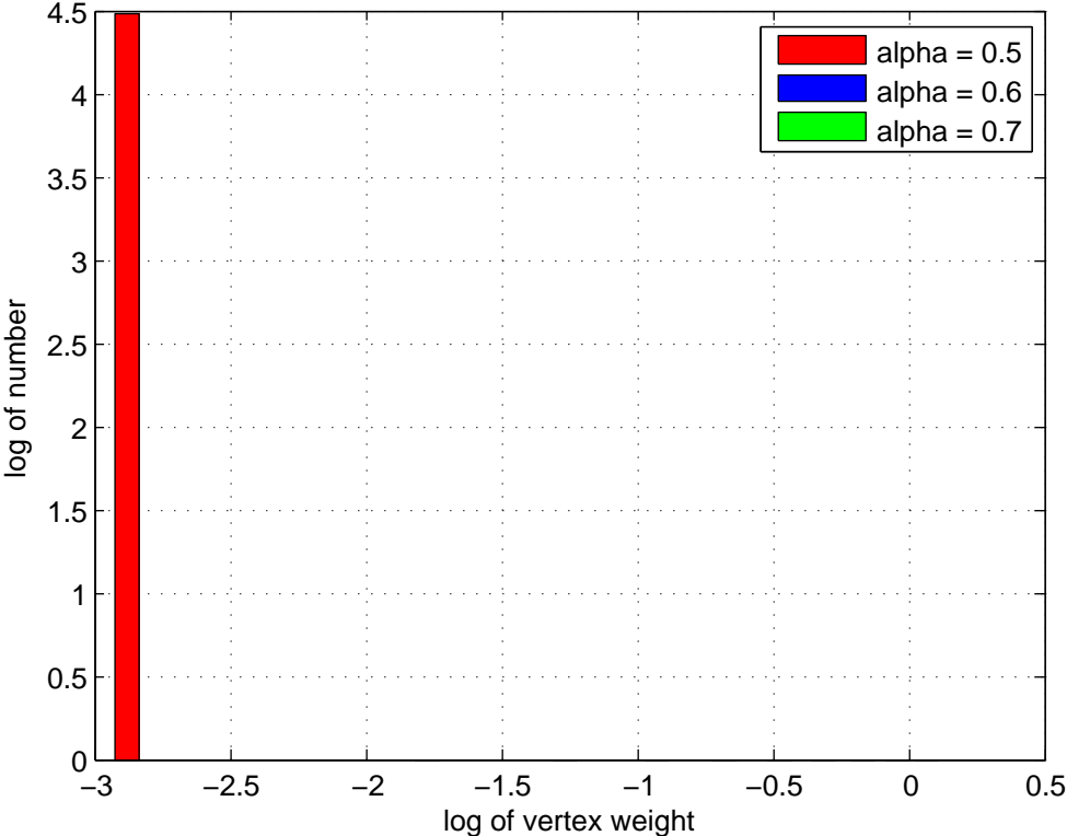
Weights of vertices in market graph (Germany 2006)
