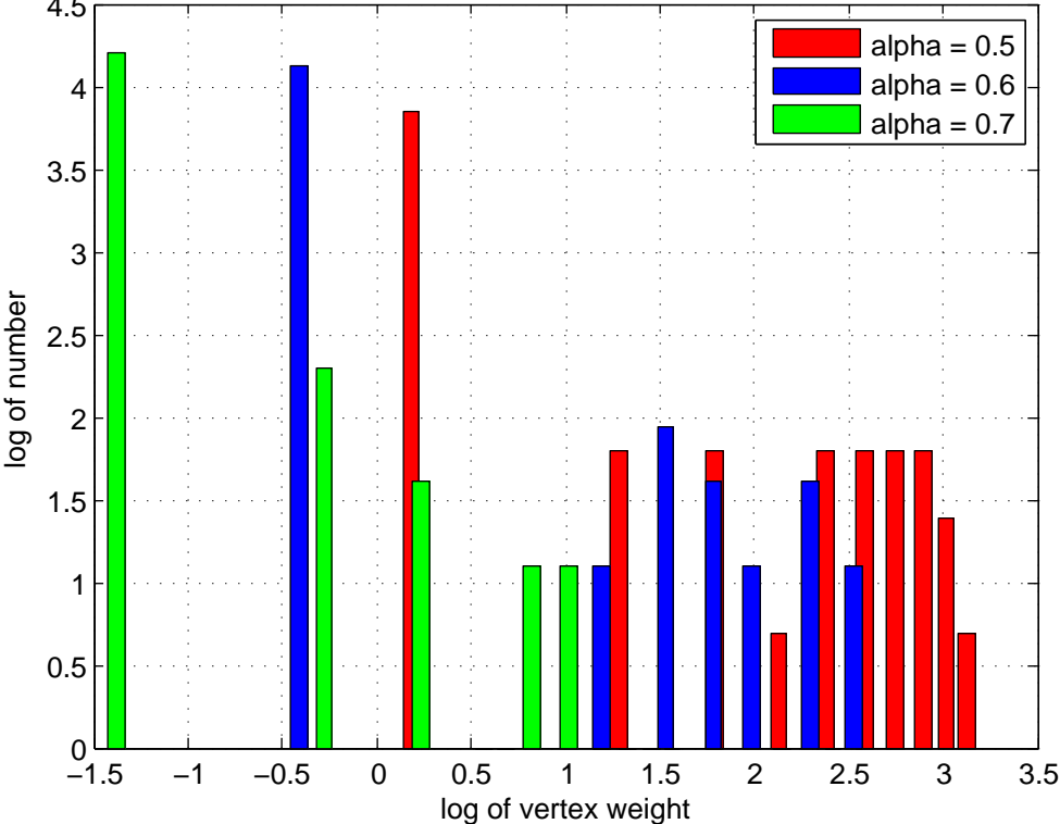
Weights of vertices in market graph (Germany 2010)
