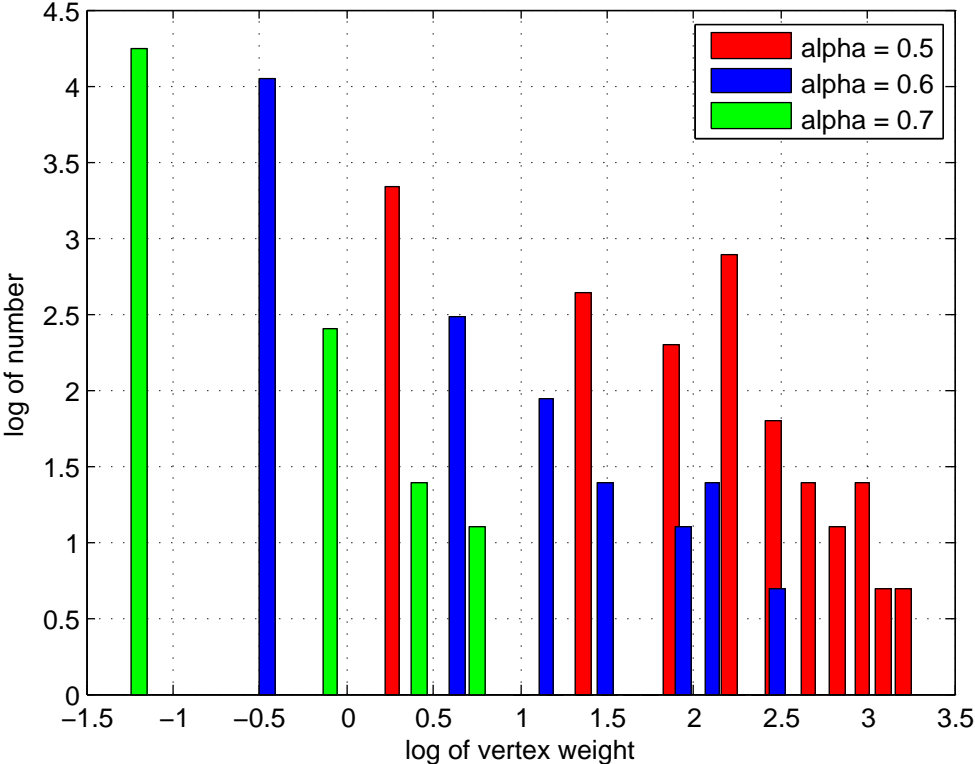
Weights of vertices in market graph (Germany 2014)
