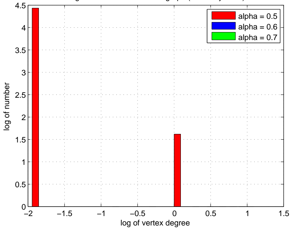
Degree of vertices in market graph (Germany 2006)
