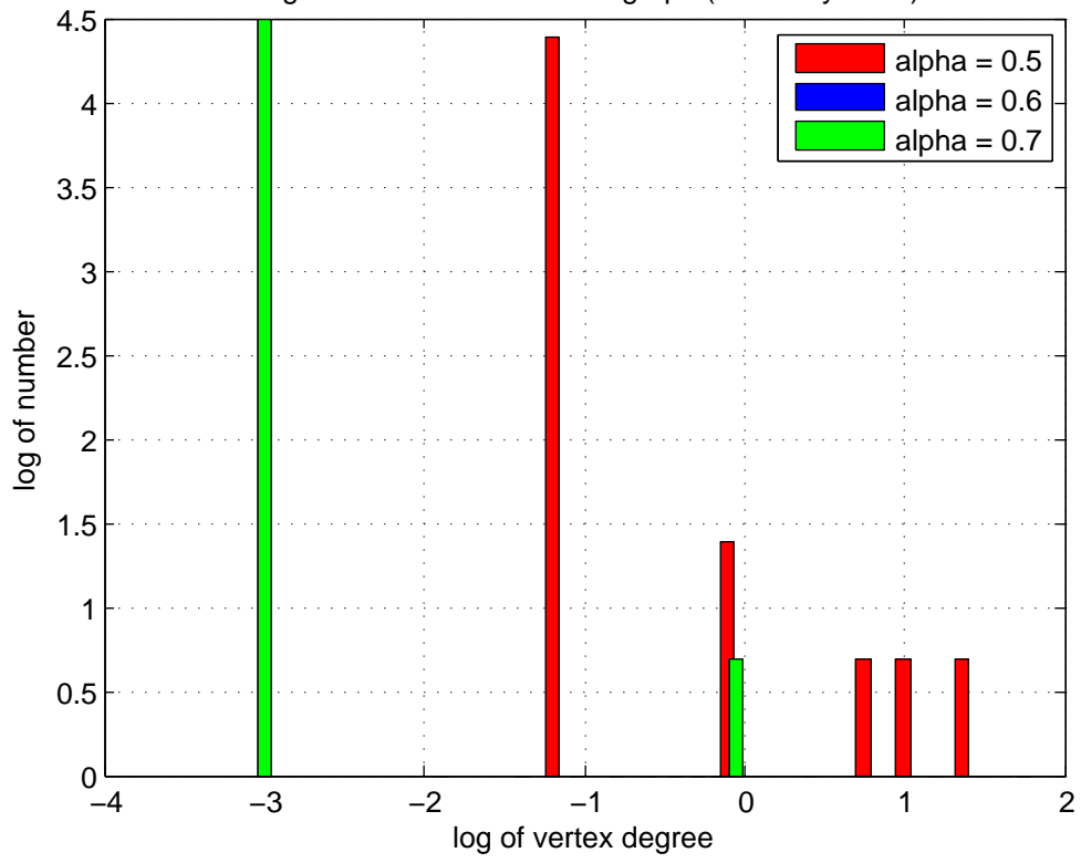
Degree of vertices in market graph (Germany 2003)
