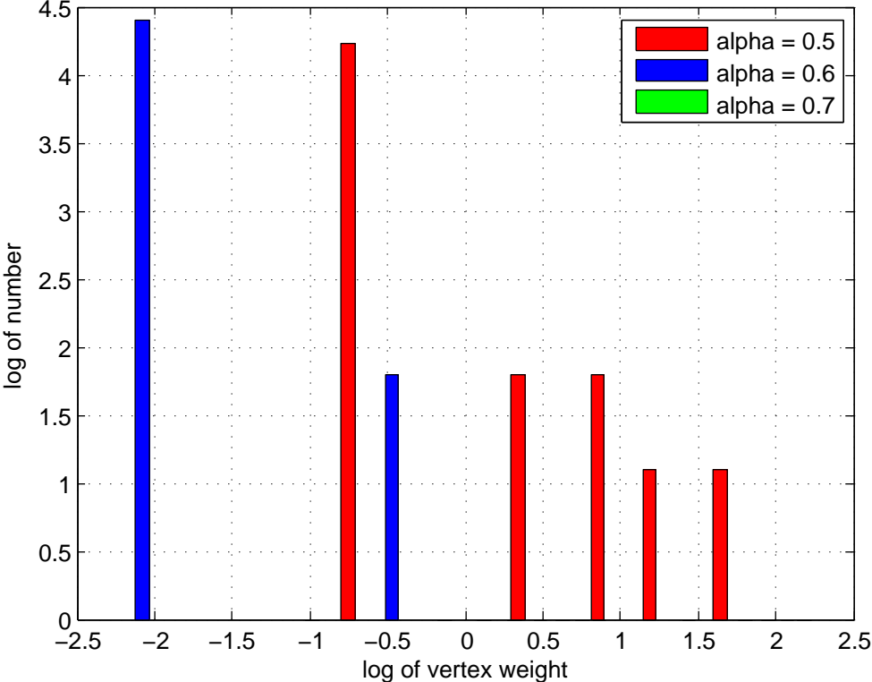
Weights of vertices in market graph (Germany 2008)
