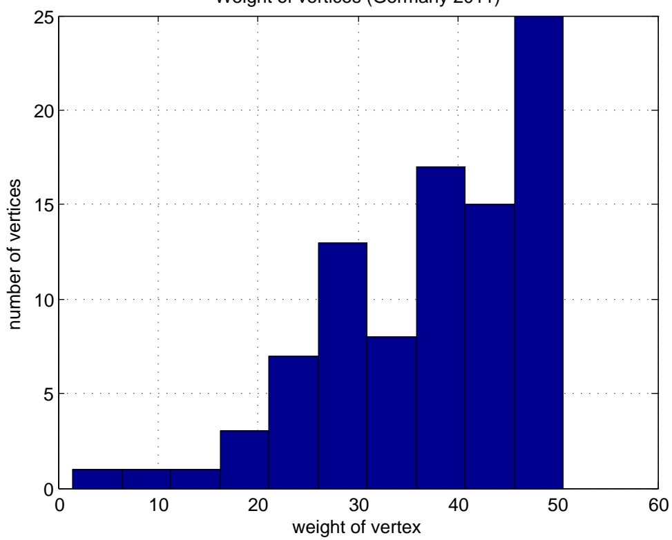
Weight of vertices (Germany 2011)
