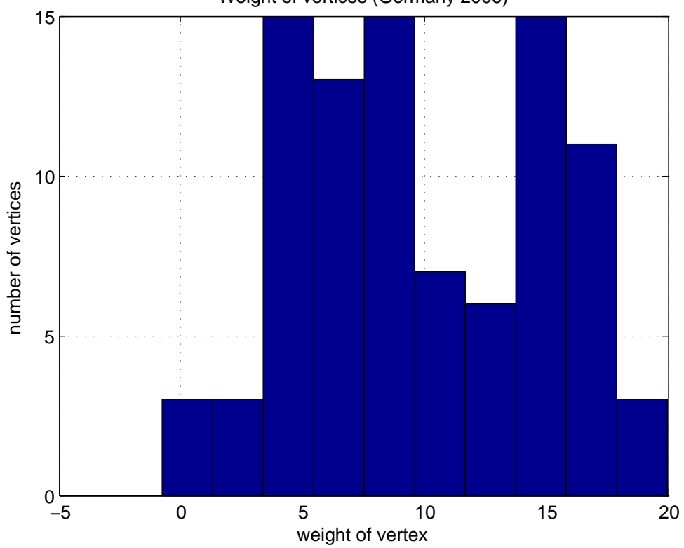
Weight of vertices (Germany 2006)
