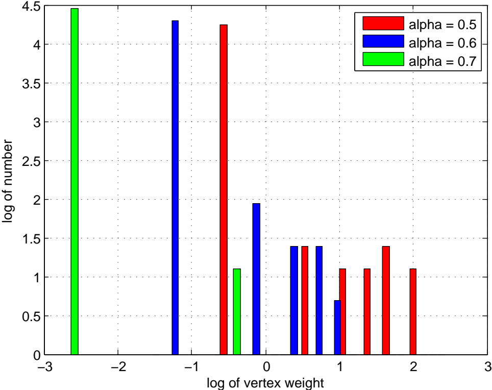
Weights of vertices in market graph (Germany 2007)
