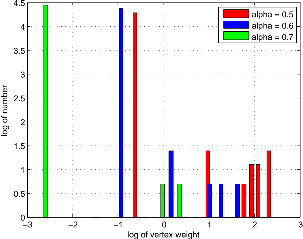
Weights of vertices in market graph (Germany 2004)
