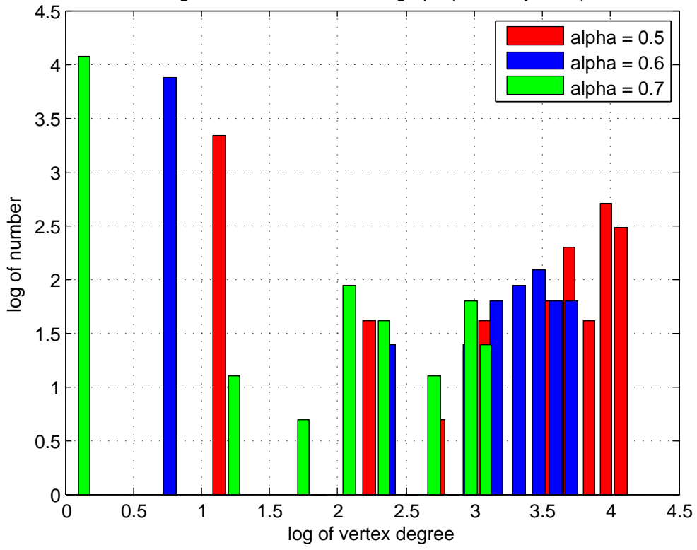
Degree of vertices in market graph (Germany 2011)
