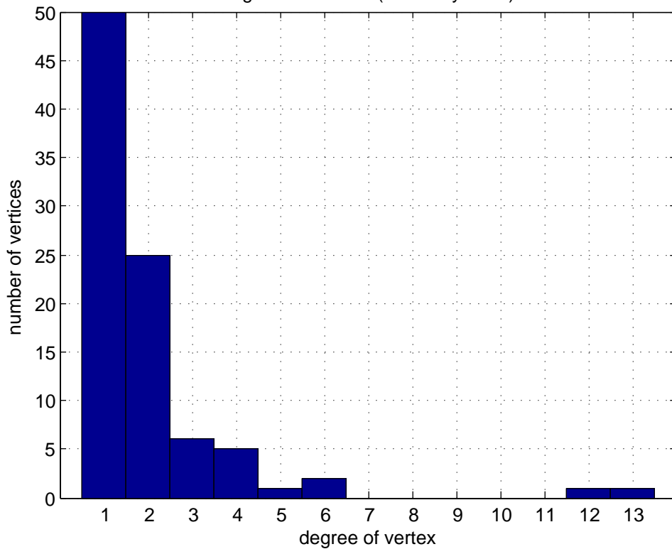
Degree of vertices (Germany 2003)
