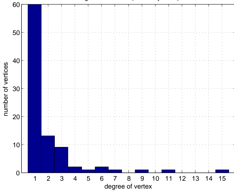
Degree of vertices (Germany 2007)
