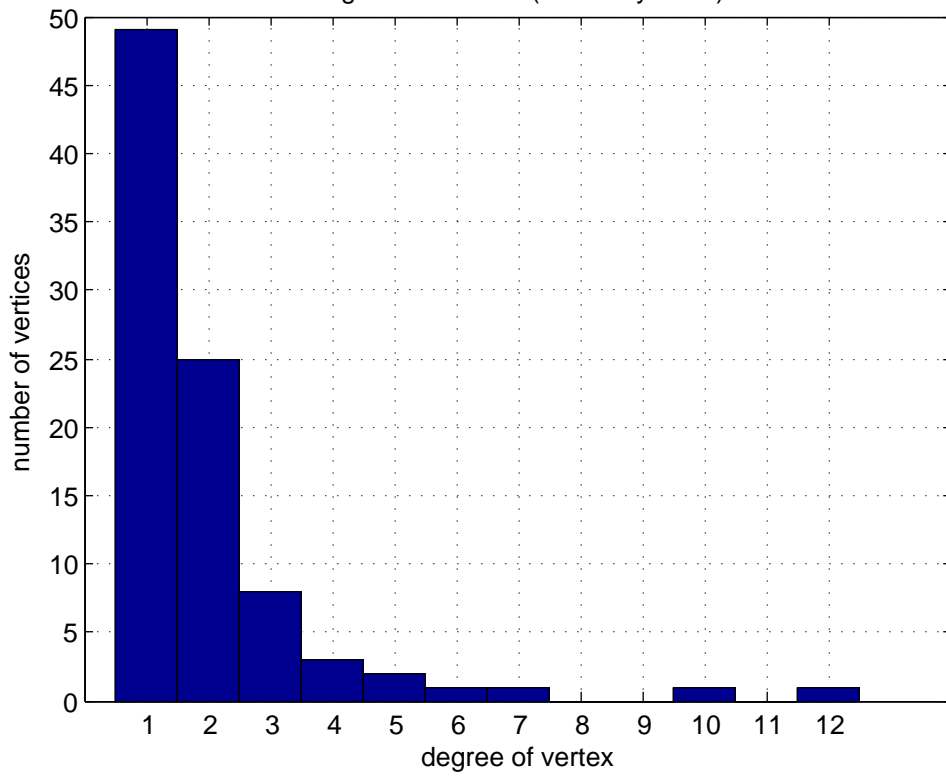
Degree of vertices (Germany 2009)
