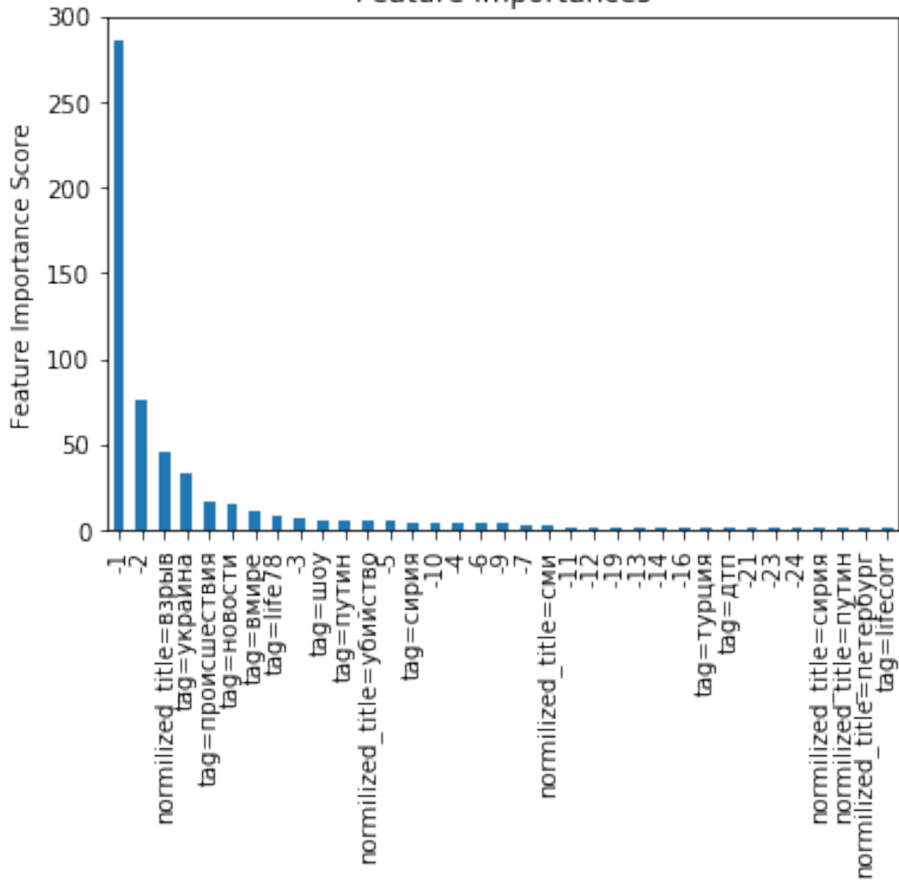
Feature Importances
